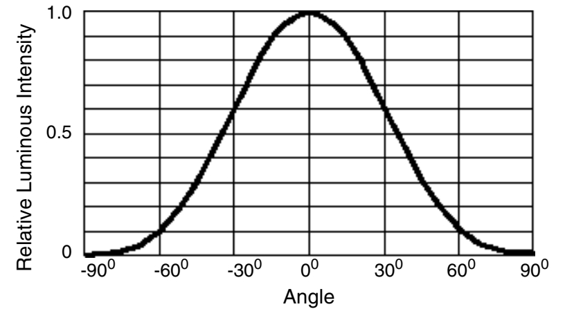
Far Field Pattern 50% Power Angle: 65°
